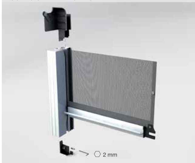
AGGANCIO INF. MANIGLIA STANDARD
